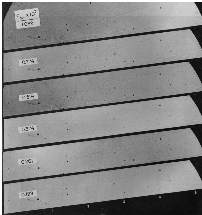
Fig. 3 Shadowgraph of instabilities with helium blown into air, from figure 3d in [12].
