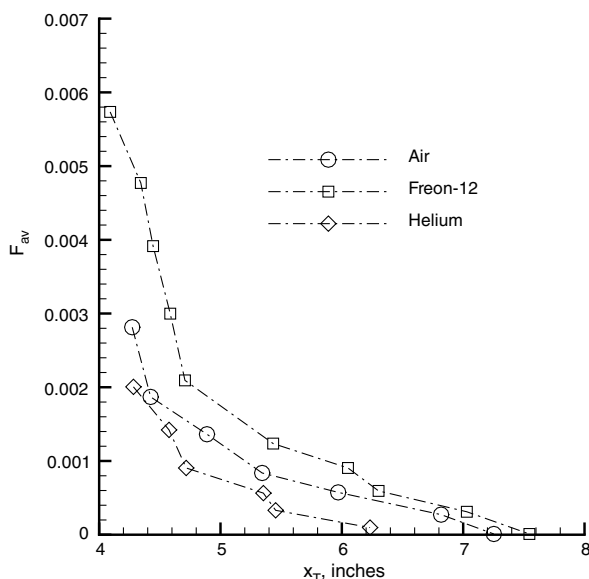
Fig. 4 Variation of transition point with injection. Sharp cone at zero AOA. Redrawn from figure 4c in [15].
